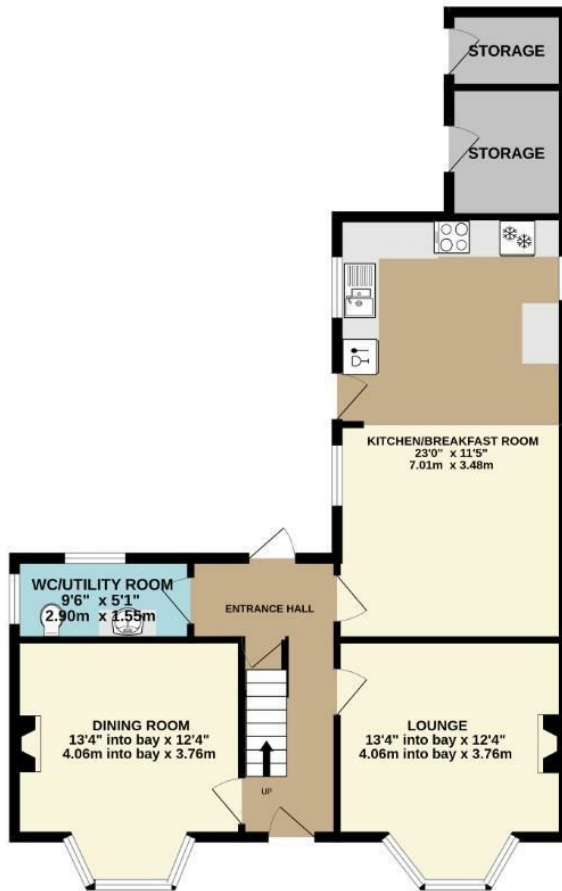
GROUND FLOOR 773 sq.ft. (71.8 sq.m.) approx.
